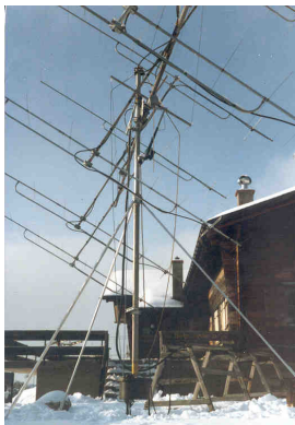
1985: the EME antenna system on "Sareiserjoch"
